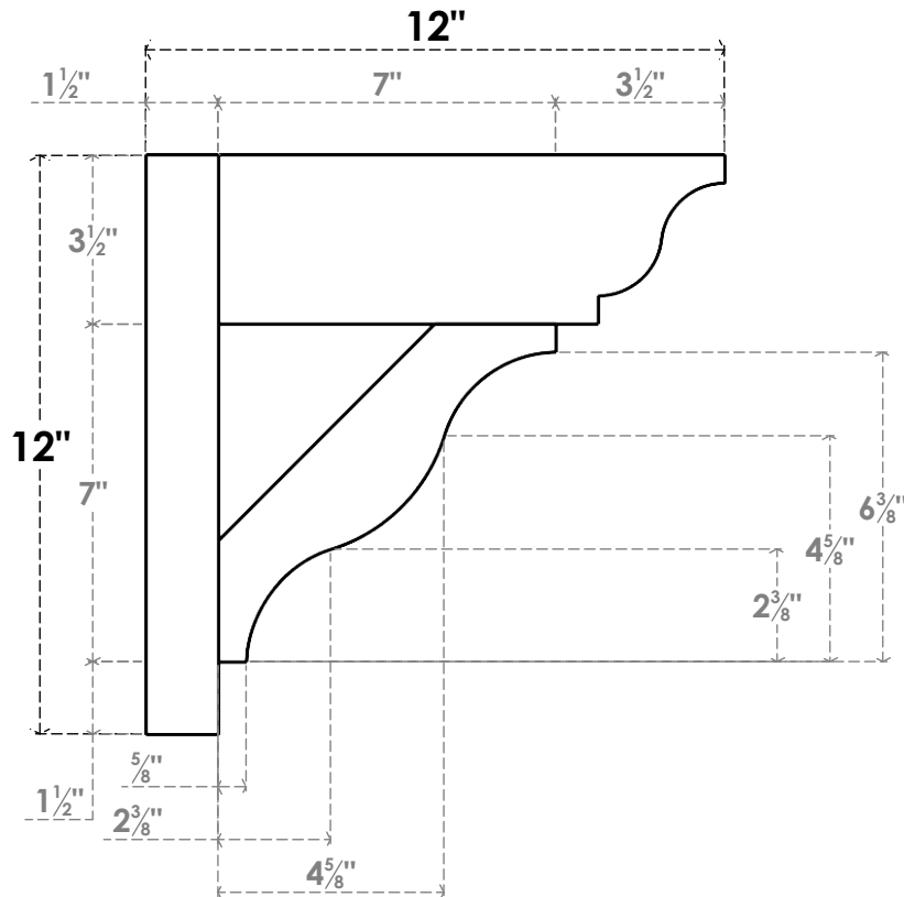
SIDE PROFILE
